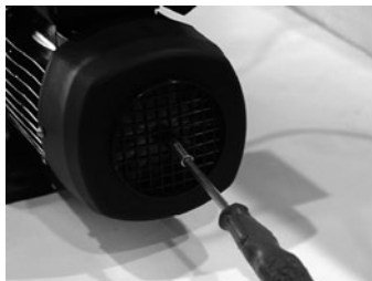
In order to avoid mechanical seal blocking, turn the shaft trough the motor fan before starting up or after extended unuse!
