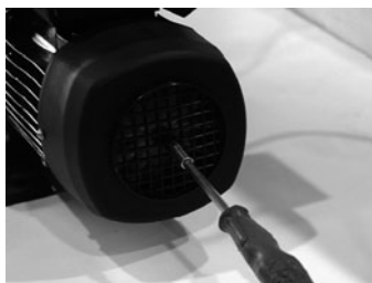
In order to avoid mechanical seal blocking, turn the shaft through the motor fan before starting up or after extended unuse!
